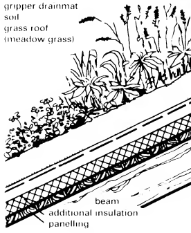
⑨ Roof cultivation on sloping roof
